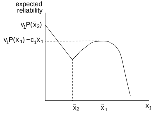
Figure 3: Sequential contribution in total efforts case.
