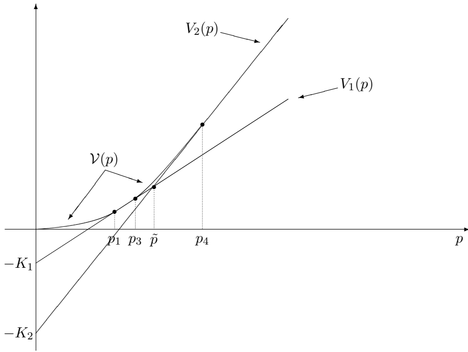
Figure 1. The value function \mathcal{V}
