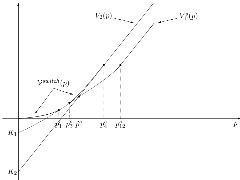
Figure 2. The value function \mathcal{V}^{switch}
